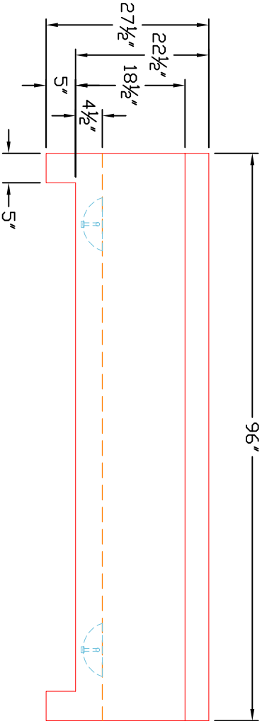
FRONT VIEW
