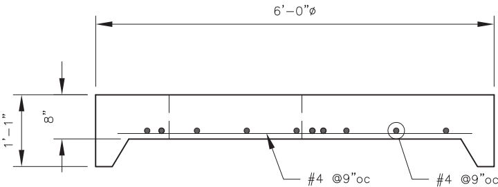
TYPICAL REINFORCING SECTION
