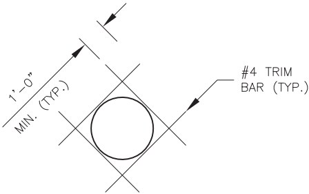
OPENING DETAIL (ROUND SHOWN, SQUARE OR RECT. SIMILAR)
