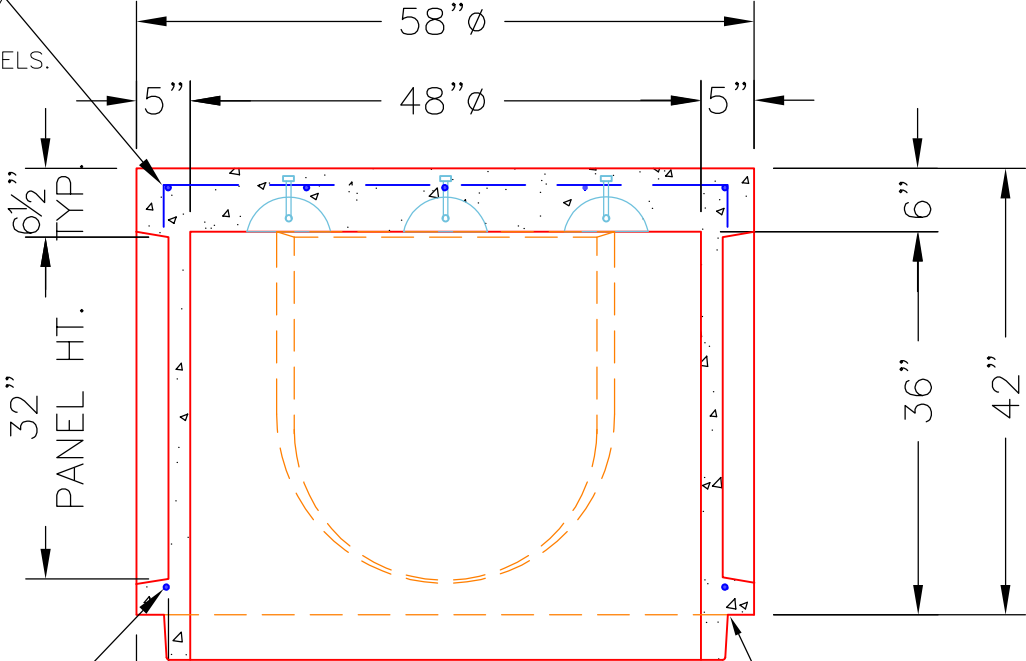
SECTION A-A (UPSIDE-DOWN)
