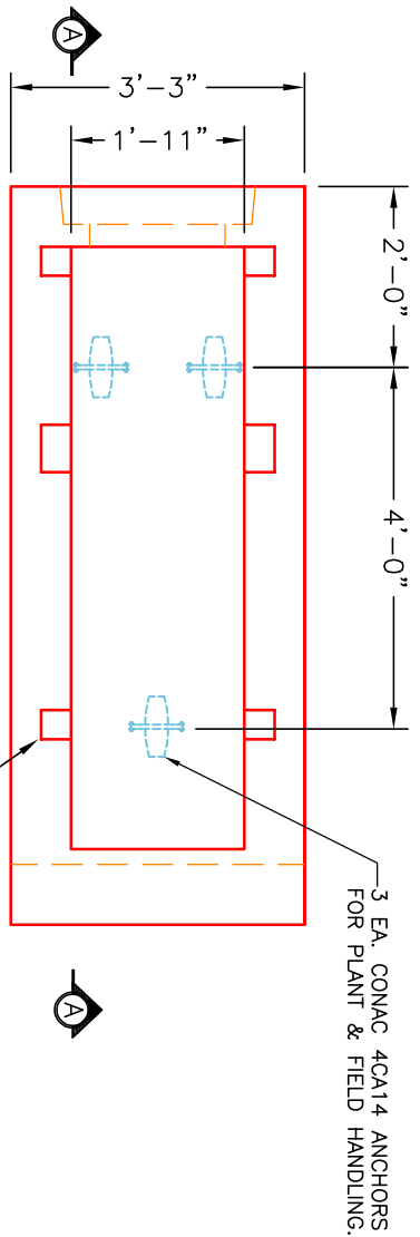
PLAN VIEW SLOTS AS REQUIRED FOR STRUCTURAL STEEL GRATES (NOT SHOWN) AS SUPPLIED BY BOTTOMS ENGINEERING OR J.R. HOE & SONS.
