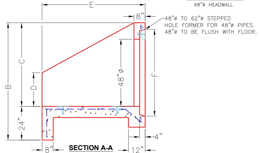
48" \phi HEADWALL
