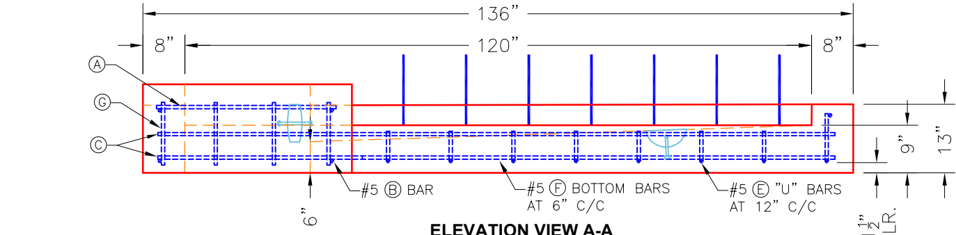
ELEVATION VIEW A-A
