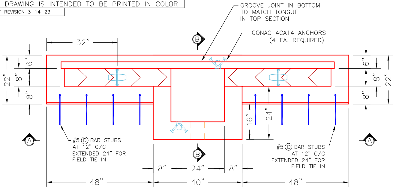
PLAN VIEW
