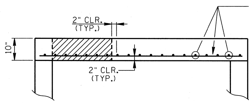
SECTION
