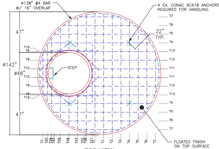
REBAR TAKEOFF (TOP LAYER)
