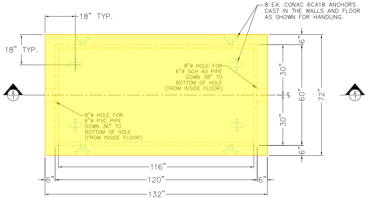
PLAN VIEW (UPSIDE-DOWN)
