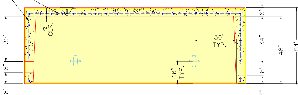
SECTION A-A (UPSIDE-DOWN)
