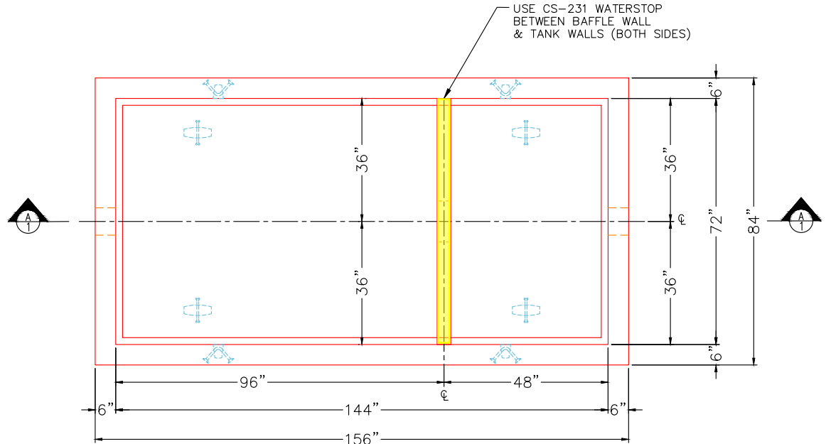
PLAN VIEW (RIGHTSIDE-UP)
