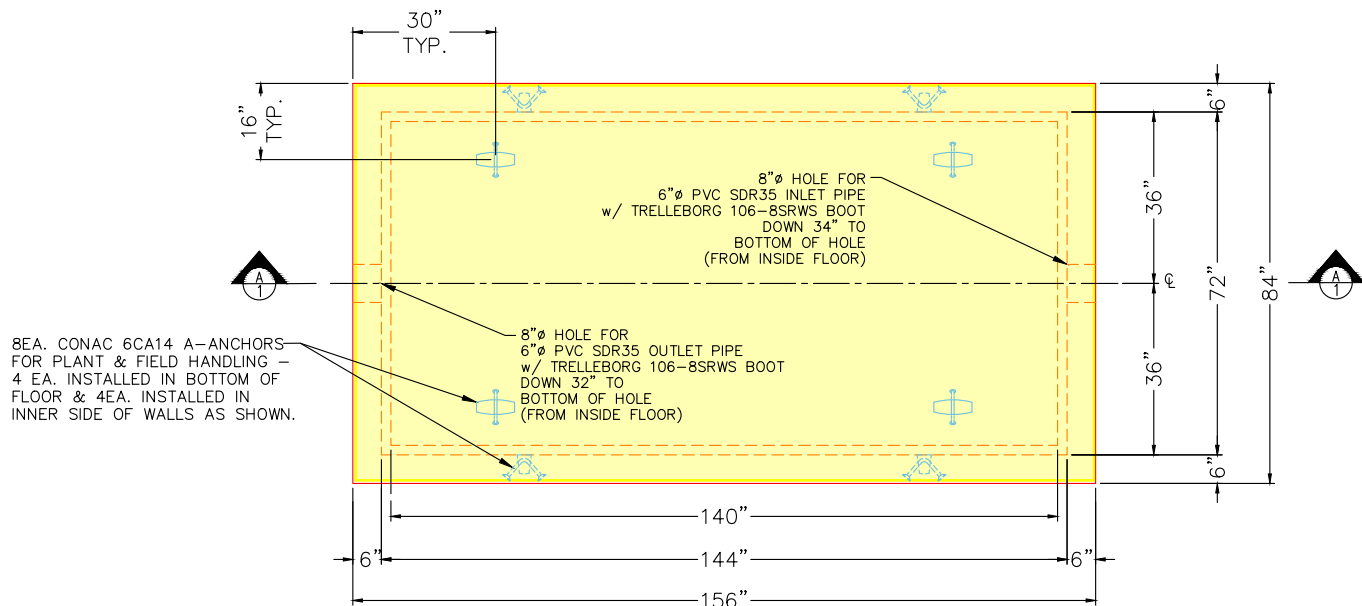
PLAN VIEW (UPSIDE-DOWN)
