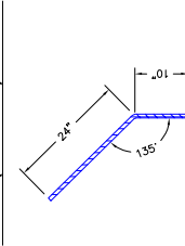
JOINT (TONGUE) DETAIL
