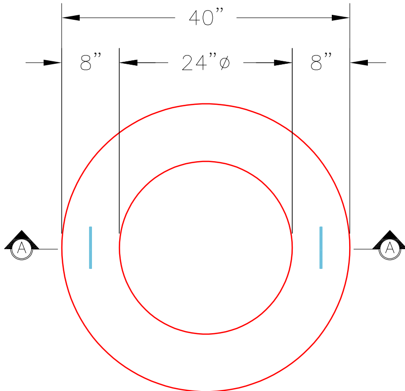
PLAN VIEW
