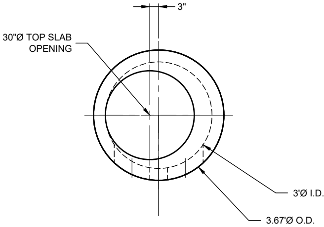
PLAN VIEW INTERNALS NOT SHOWN
