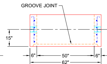
SIDE VIEW (RIGHT SIDE UP)
