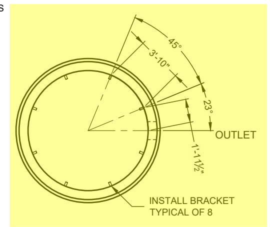
SUPPORT BRACKET LAYOUT PLAN VIEW
