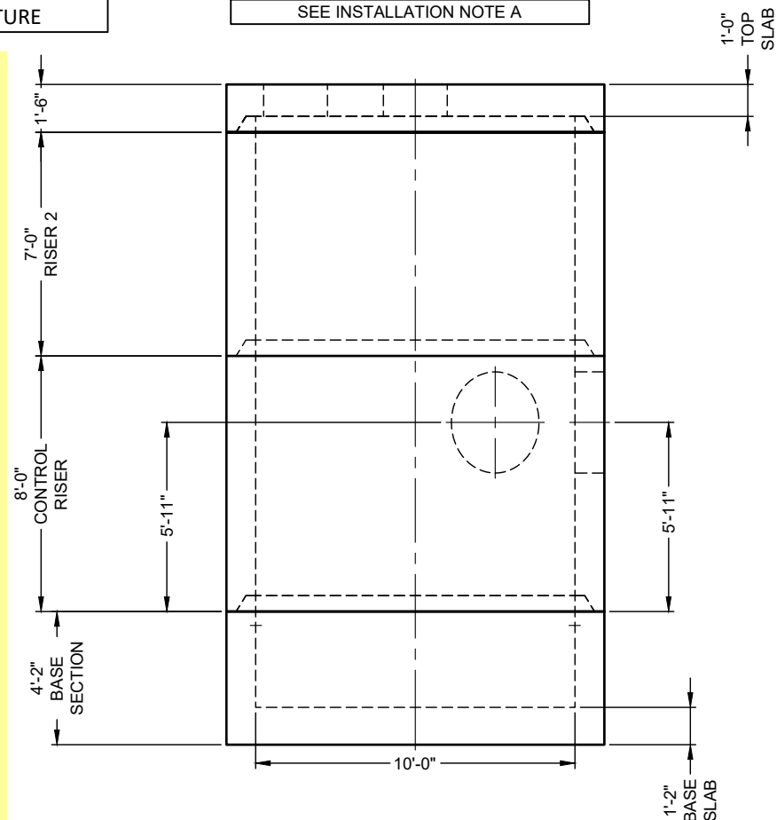
PRECAST COMPONENTS INTERNALS NOT SHOWN
