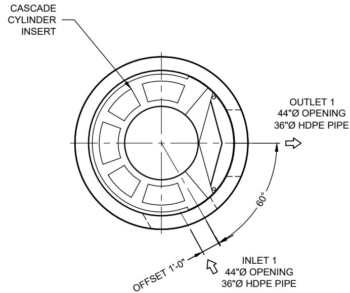
PLAN VIEW FOR PIPE ORIENTATION TOP SLAB NOT SHOWN
