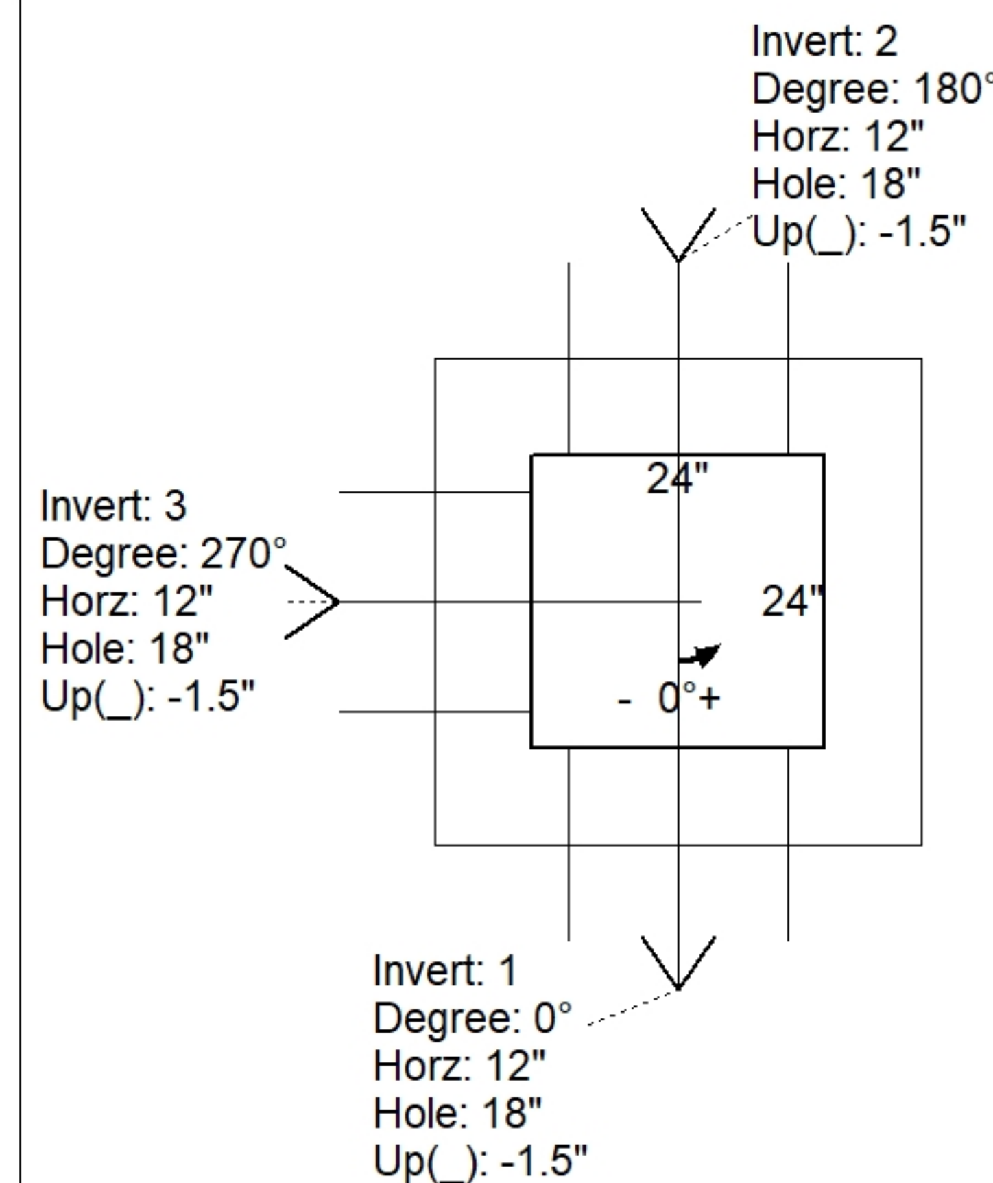
UPSIDE-DOWN VIEW (int. dimensions)
