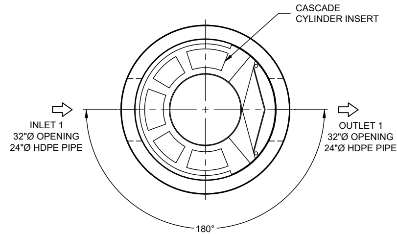
PLAN VIEW FOR PIPE ORIENTATION
