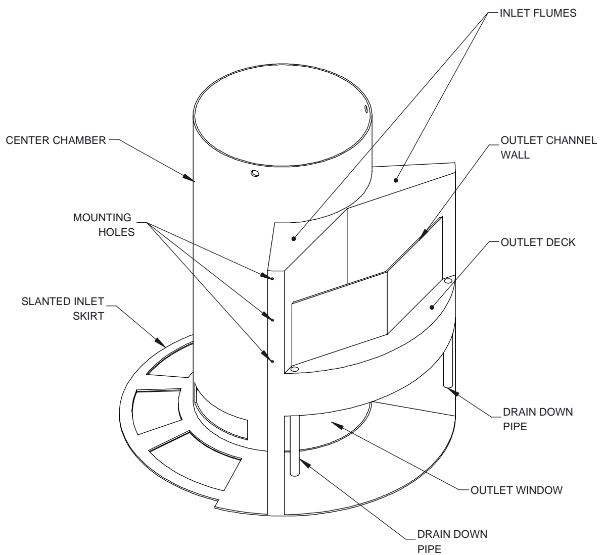
ISOMETRIC VIEW
