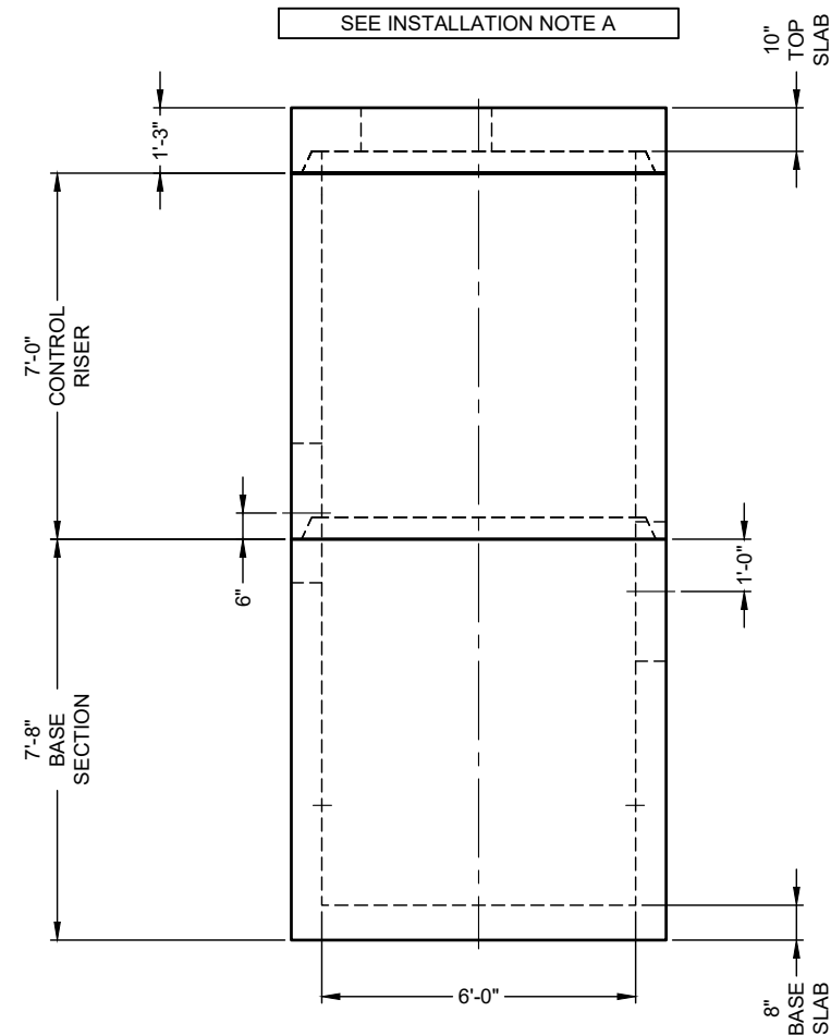
PRECAST COMPONENTS
