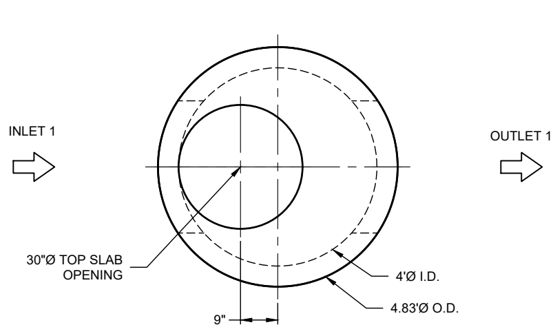
PLAN VIEW INTERNALS NOT SHOWN
