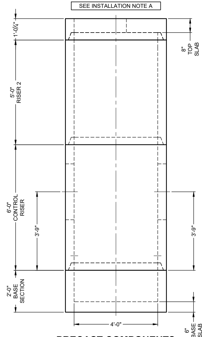
PRECAST COMPONENTS INTERNALS NOT SHOWN
