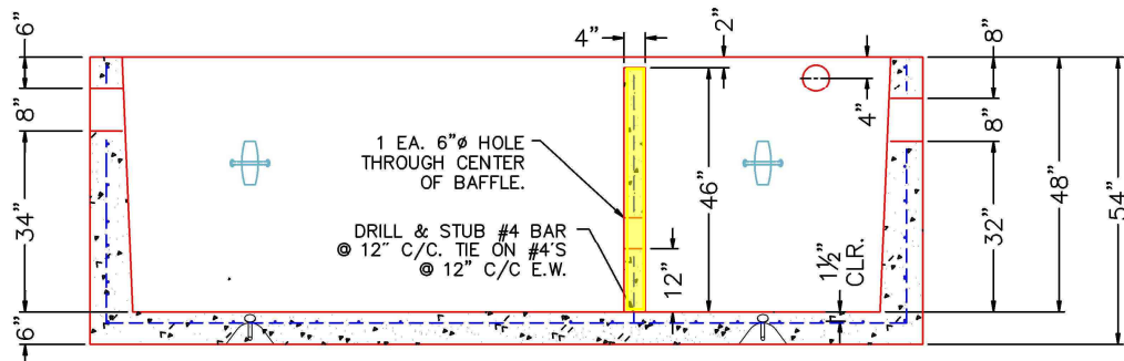
SECTION A-A (RIGHTSIDE-UP)
