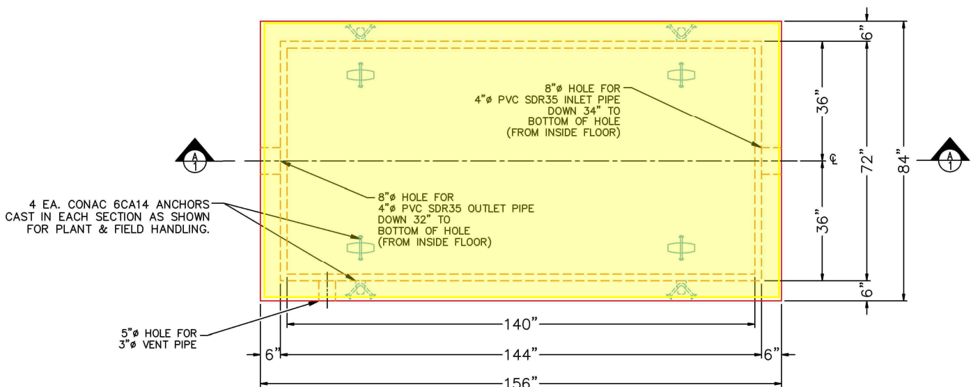
PLAN VIEW (UPSIDE-DOWN)
