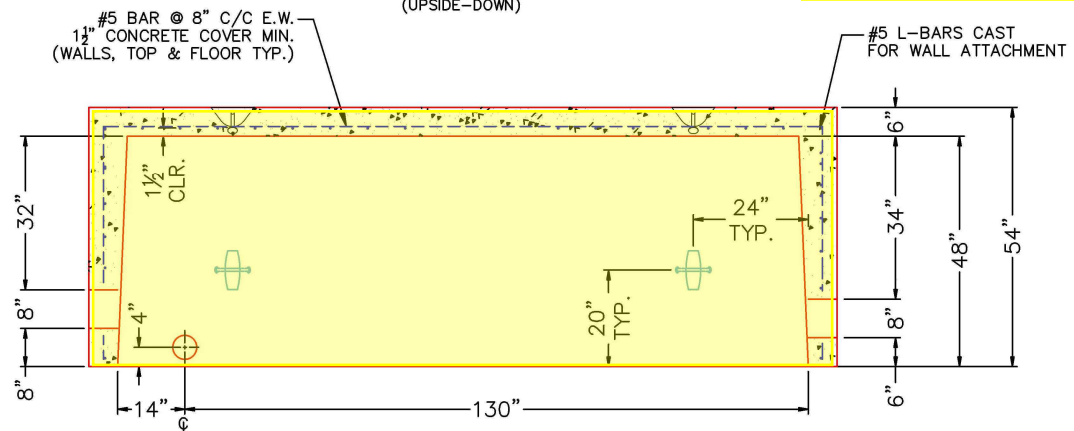
SECTION A-A (UPSIDE-DOWN)
