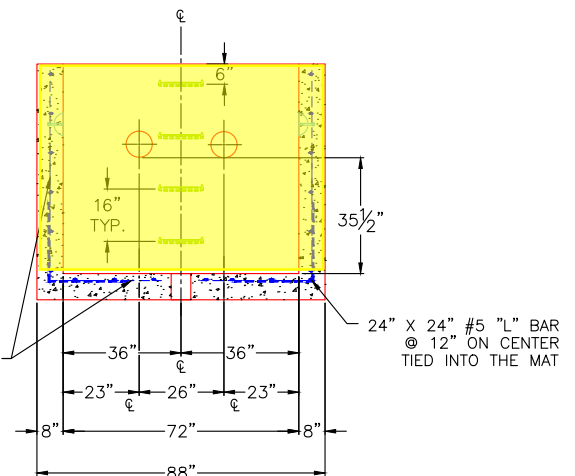
SECTION B-B (RIGHT-SIDE-UP VIEW)
