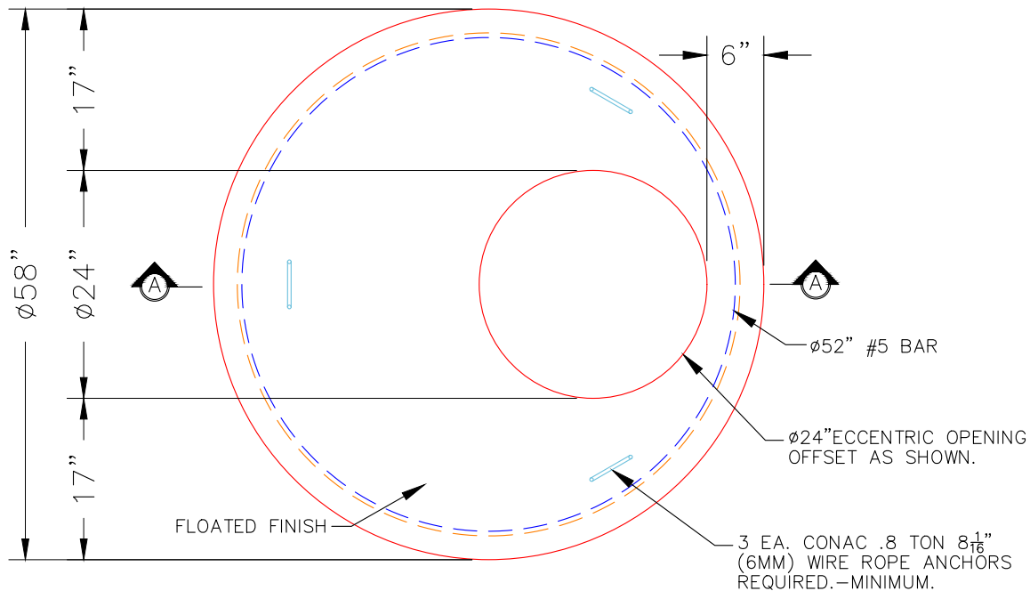
PLAN VIEW
