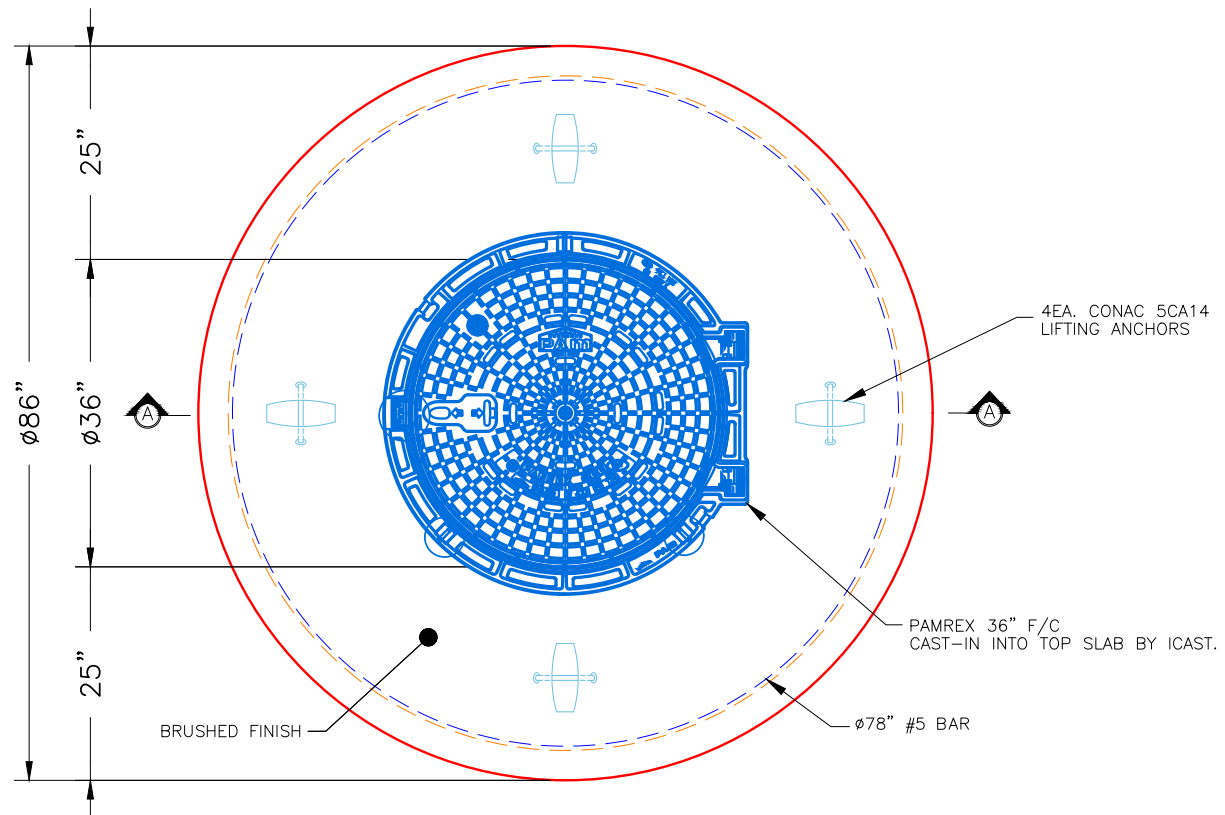
PLAN VIEW
