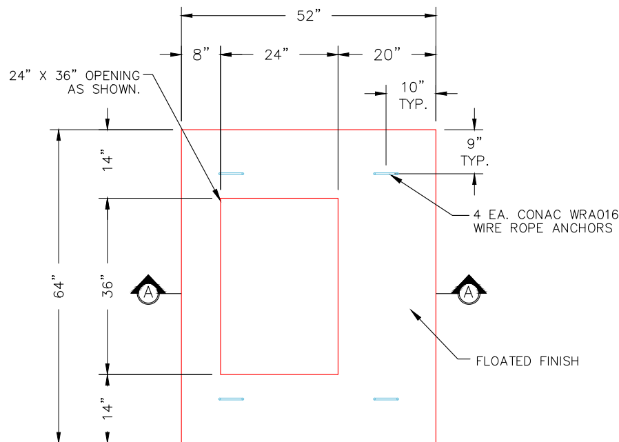
PLAN VIEW
