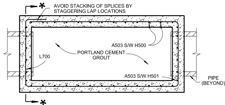
SECTION E-E
