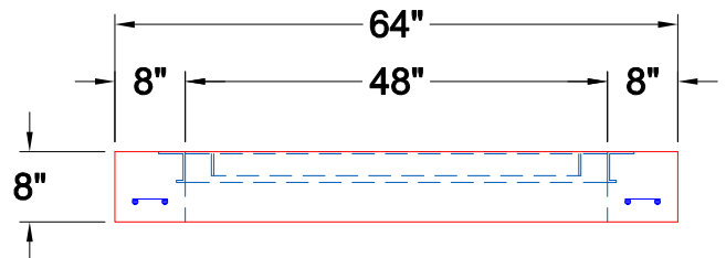
RIGHT VIEW
