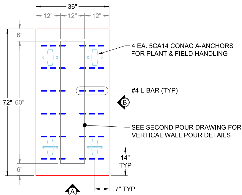
PLAN VIEW (RIGHT SIDE UP)
