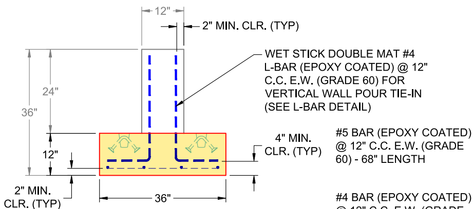
VIEW A (RIGHT SIDE UP)
