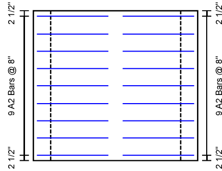
Bottom Slab Corner Reinf.
