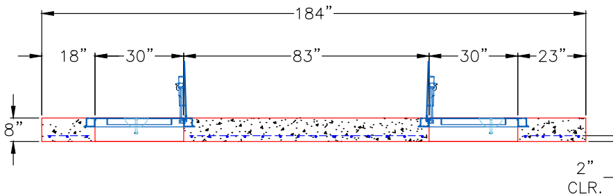
SECTION A-A (RIGHT-SIDE-UP VIEW)
