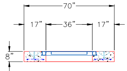
SECTION B-B (RIGHT-SIDE-UP VIEW)
