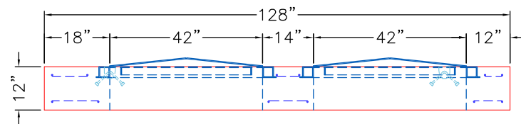
RIGHT VIEW
