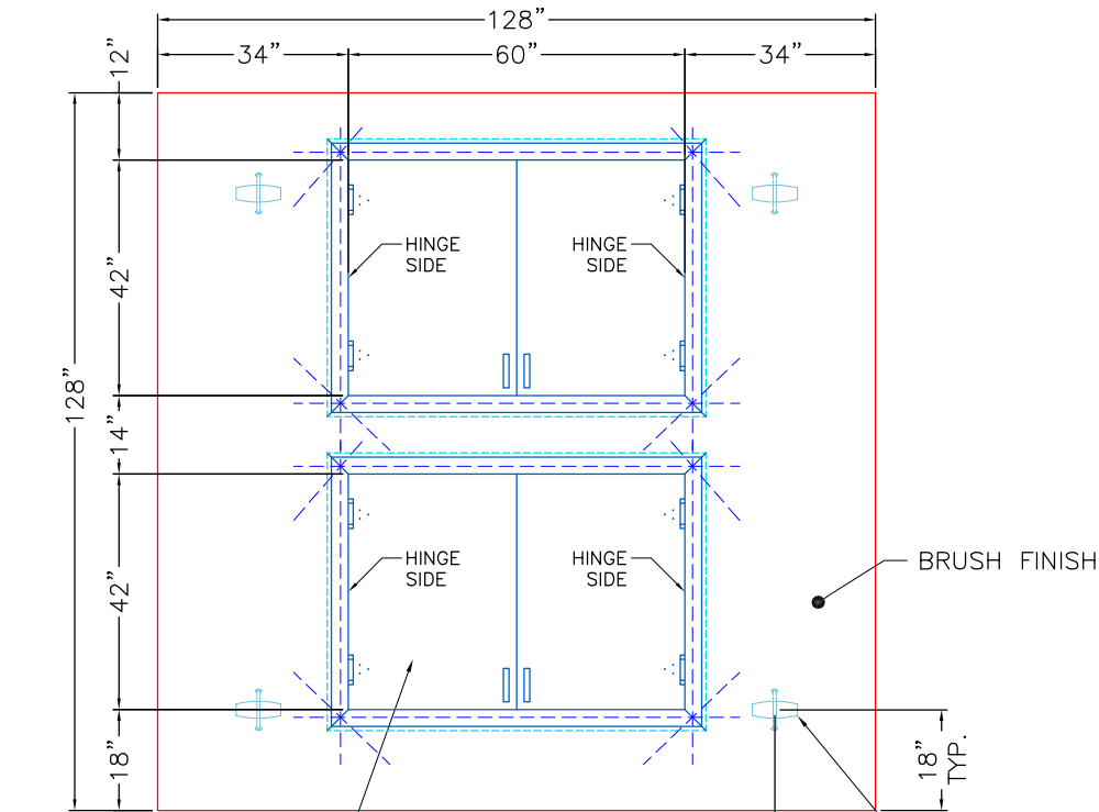
PLAN VIEW
