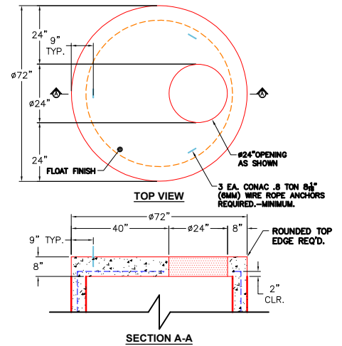
RIGHT-SIDE UP VIEW (MONOTOP)
