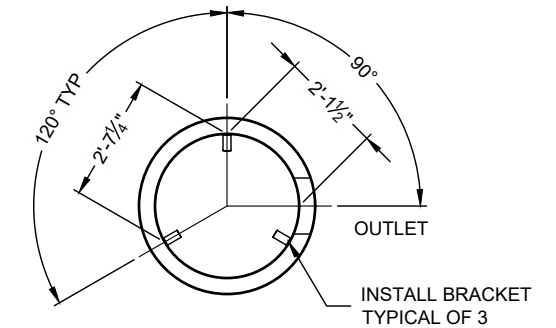
SUPPORT BRACKET LAYOUT PLAN VIEW
