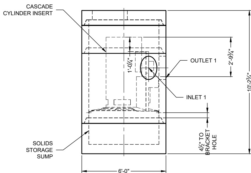
ELEVATION VIEW
