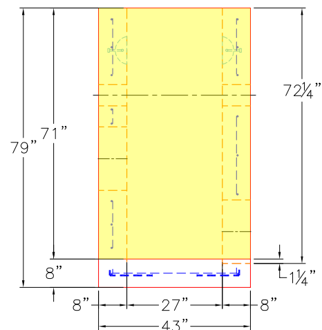
RIGHT VIEW
