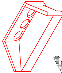
ISOMETRIC VIEW TRIPLE 36" EQ. HW SHOWN
