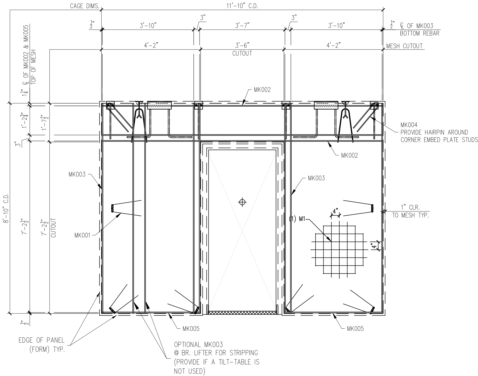
NORTH WALL REINFORCING SCALE: \frac{1}{2}'' = 1'-0''
