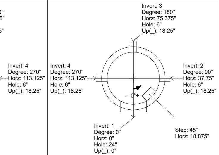
UPSIDE-DOWN VIEW (int. dimensions)
