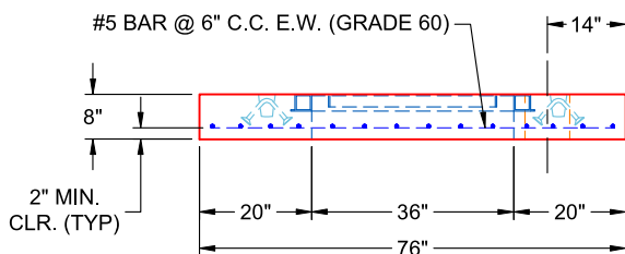
FRONT VIEW (RIGHT SIDE UP)
