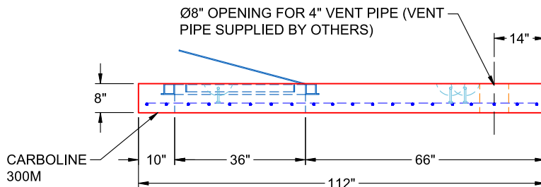
SIDE VIEW (RIGHT SIDE UP)
