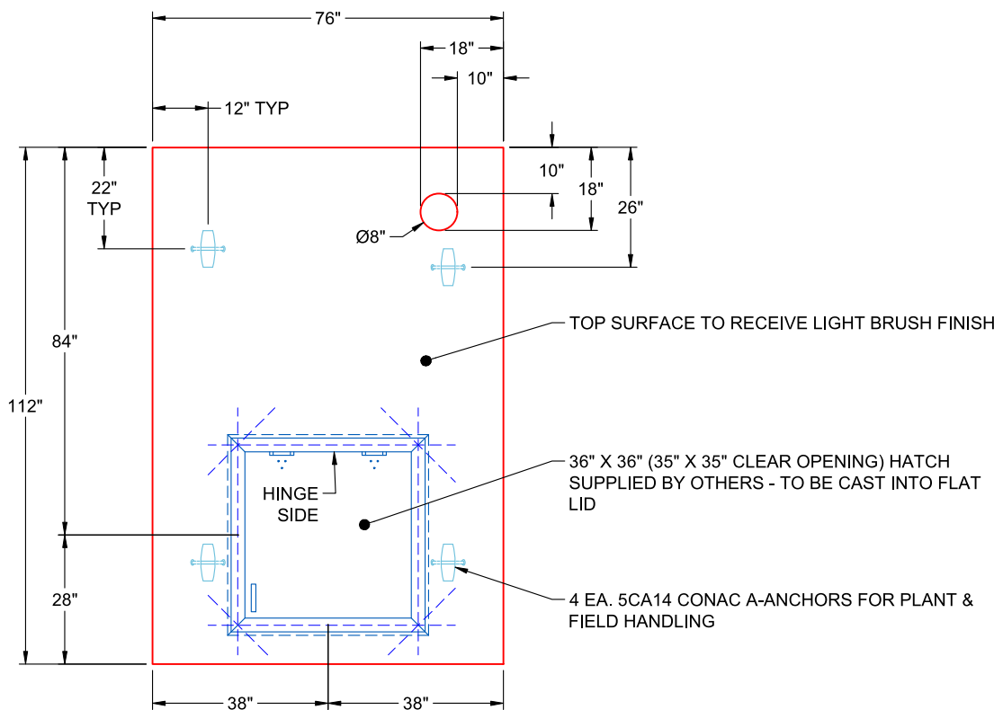
PLAN VIEW (RIGHT SIDE UP)
