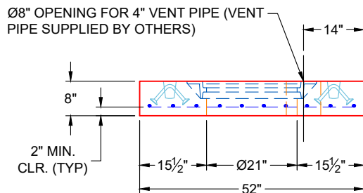
FRONT VIEW (RIGHT SIDE UP)
