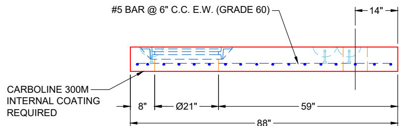
SIDE VIEW (RIGHT SIDE UP)
