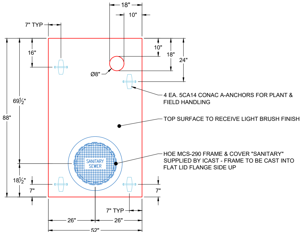
PLAN VIEW (RIGHT SIDE UP)
