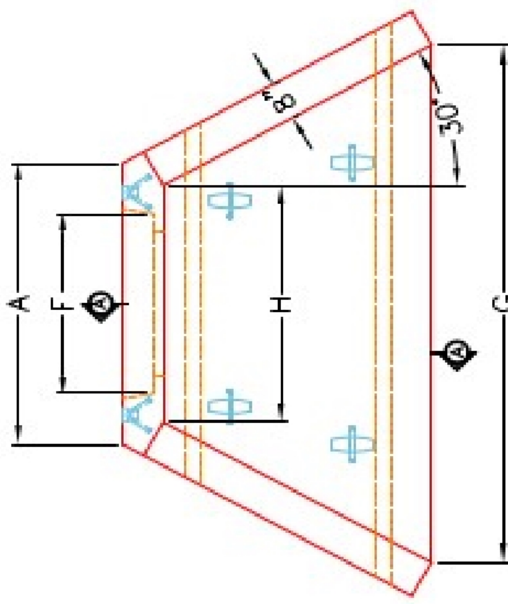
PLAN VIEW
