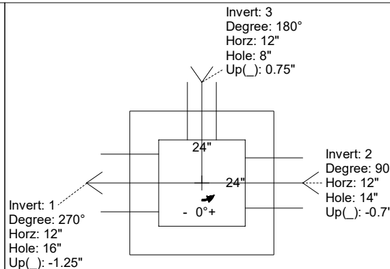
UPSIDE-DOWN VIEW (int. dimensions)
