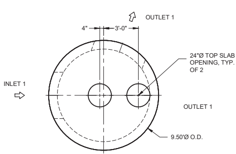
PLAN VIEW INTERNALS NOT SHOWN
