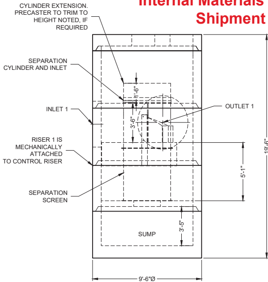
ELEVATION VIEW
