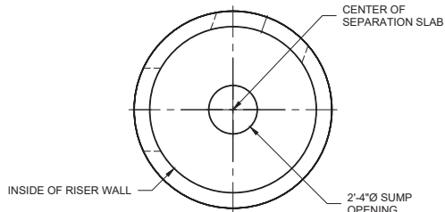
SEPARATION SLAB
