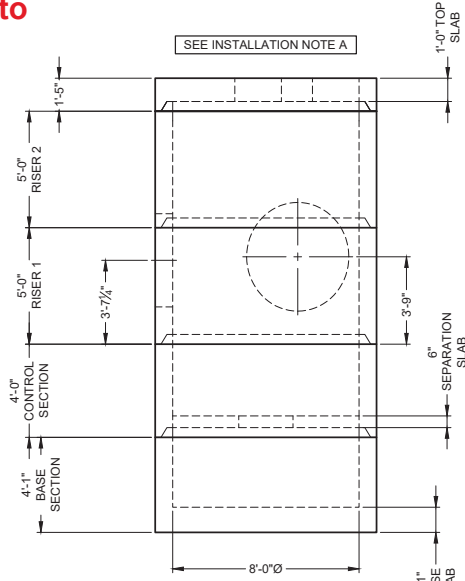
PRECAST COMPONENTS INTERNALS NOT SHOWN
