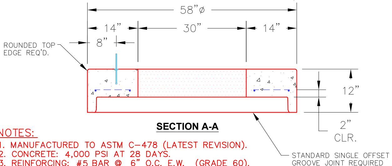
PLAN VIEW
