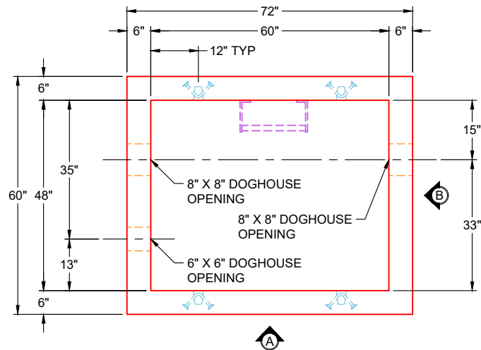
PLAN VIEW (RIGHT SIDE UP)
