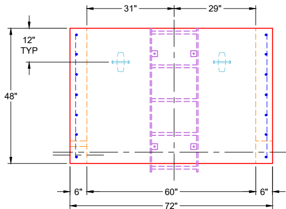
VIEW A (RIGHT SIDE UP)
