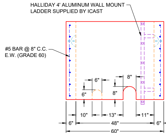
VIEW B (RIGHT SIDE UP)
