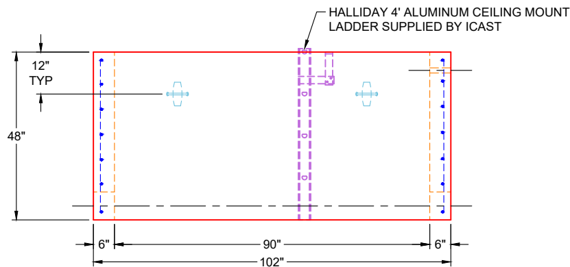
VIEW A (RIGHT SIDE UP)
