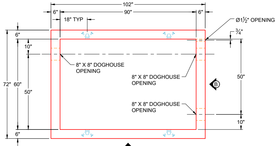
PLAN VIEW (RIGHT SIDE UP)
