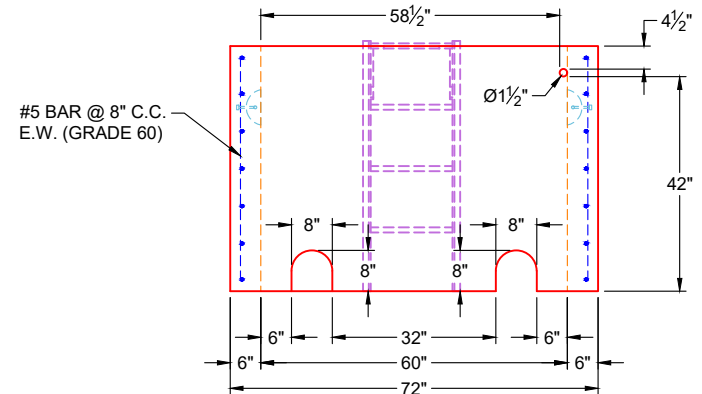
VIEW B (RIGHT SIDE UP)
