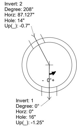
UPSIDE-DOWN VIEW (int. dimenions)
