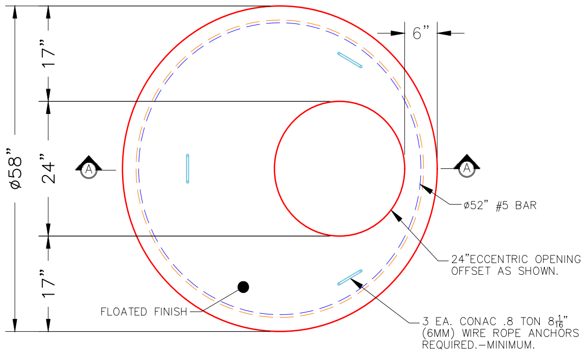
PLAN VIEW
