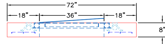
SECTION B-B
