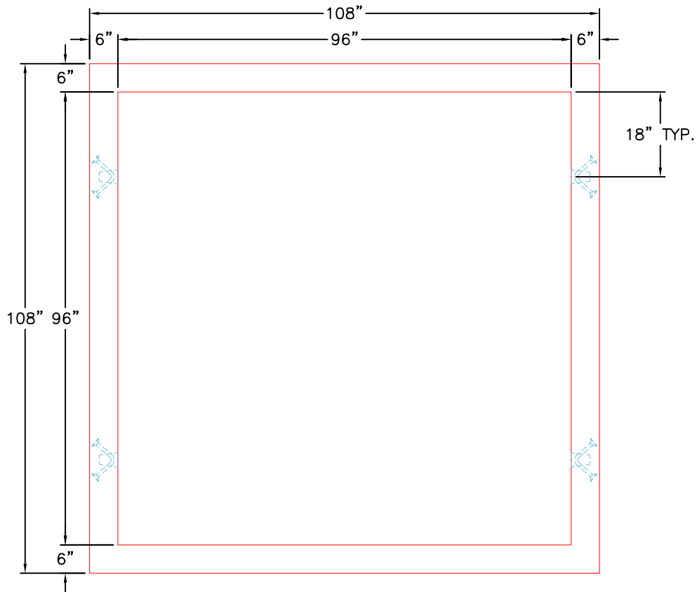
TOP VIEW
